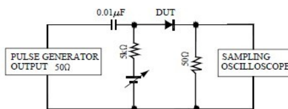
Reverse Recovery Time Measurement Circuit
