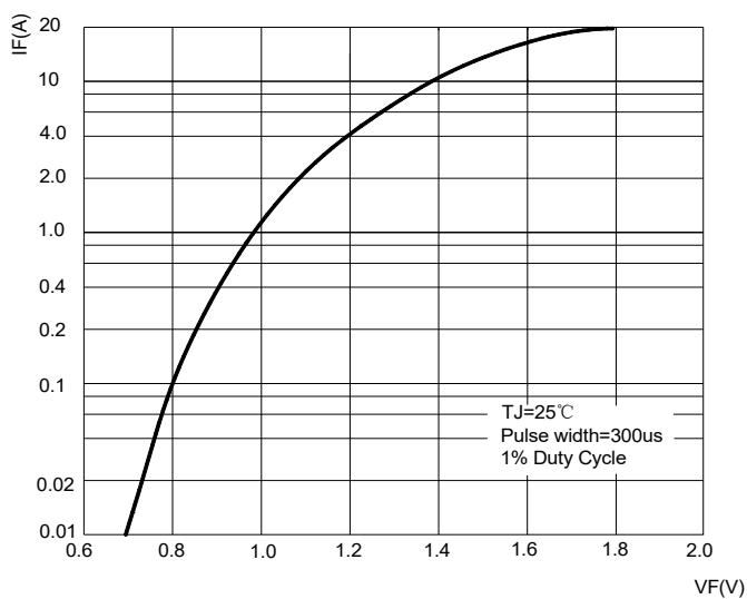
FIG.3: Forward Voltage
